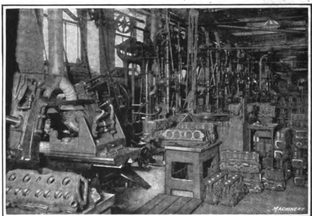
Fig. 13—In the cylinder department of the Cadillac Motor Car Co. there is a stand between each pair of machines, of the same height as the machine tables, so the operator does not have to stoop. Castings are swung from machine to stand and thence to next machine
